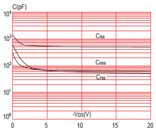
Figure 6: Capacitance Characteristics
