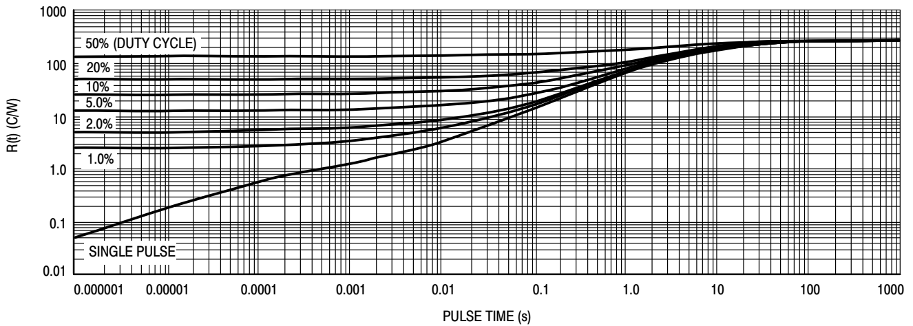
Figure 8. Thermal Response, Junction-to-Ambient ( 6\text{ mm}^2 pad)
