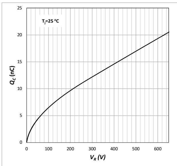
Fig. 7 Capacitive Charge
