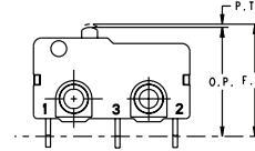
Operate Point References for PCB Terminals
