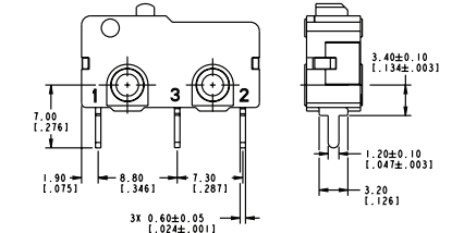
Terminal Type 20 - Straight PCB
