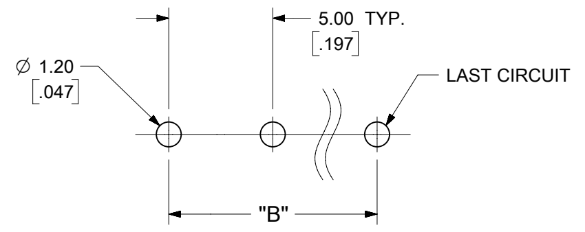
PCB LAYOUT
