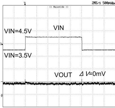
Fig.58 Transient_response (Ta=-40°C)
