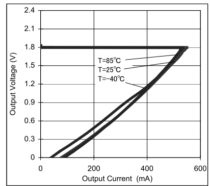
Fig.6 OCP Threshold
