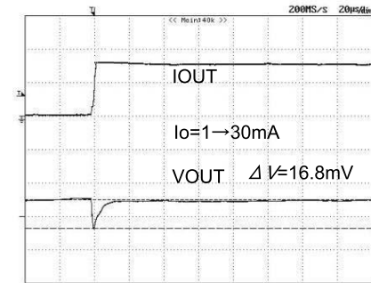
Fig.43 Load_response (Io=1→30mA) (Ta=85°C)
