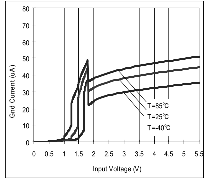
Fig.3 Circuit Current
