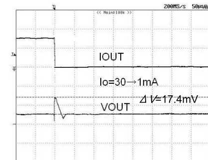
Fig.46 Load_response (Io=30→1mA) (Ta=85°C)
