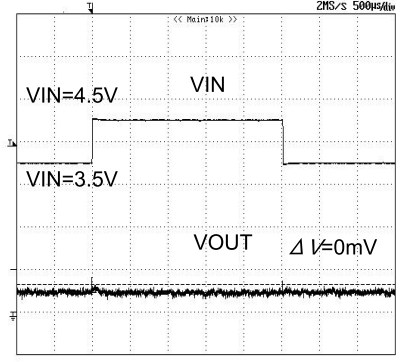
Fig.60 Transient_response (Ta=85°C)
