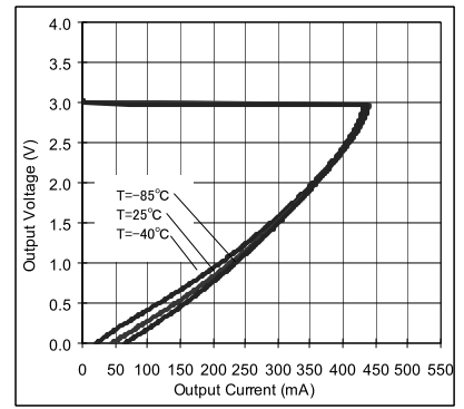
Fig.52 OCP Threshold
