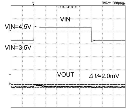
Fig.14 Transient_response (Ta=85°C)
