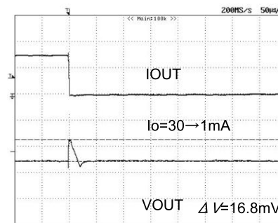
Fig.68 Load_response (Ta=25°C) (Io=30→1mA)
