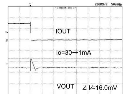
Fig.69 Load_response (Ta=85°C) (Io=30→1mA)
