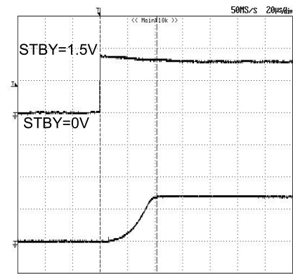
Fig.40 START_UP (Ta=85°C)
