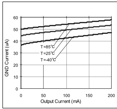
Fig.51 IOUT - IGND
