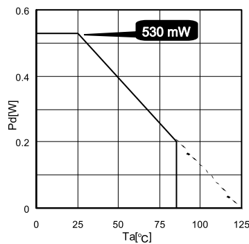
Fig.71 VCSP60N1 Power Dissipation/Power Dissipation Reduction (Example)
