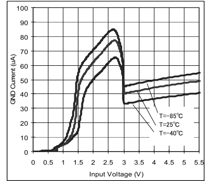
Fig.49 Circuit Current
