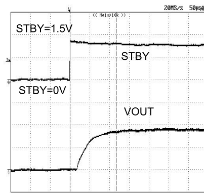
Fig.16 START_UP (Ta=25°C)
