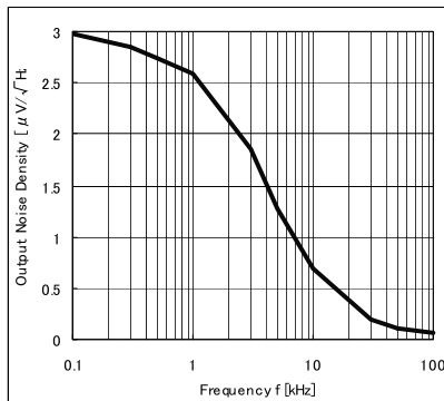
Fig.11 Noise - Freq.
