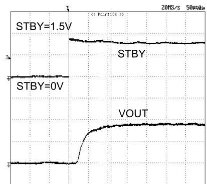
Fig.17 START_UP (Ta=85°C)
