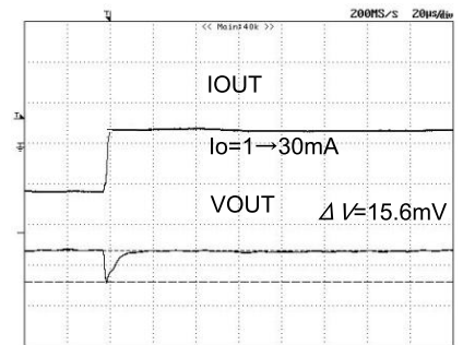
Fig.66 Load_response (Ta=85°C) (Io=1→30mA)
