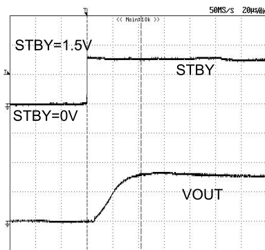
Fig.61 START_UP (Ta=-40°C)
