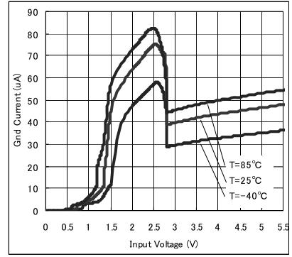
Fig.26 Circuit Current
