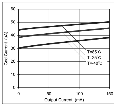
Fig.5 IOUT - IGND
