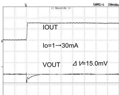
Fig.18 Load_response (Io=1→30mA) (Ta=-40°C)
