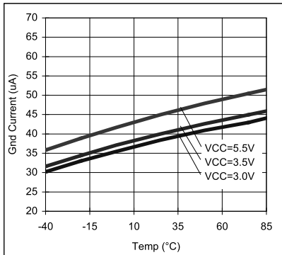
Fig.8 IGND - Temp
