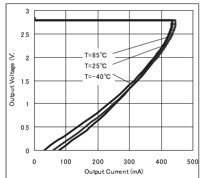
Fig.29 OCP Threshold
