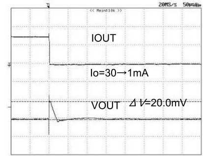
Fig.23 Load_response (Io=30→1mA) (Ta=85°C)
