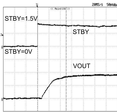
Fig.15 START_UP (Ta=-40°C)
