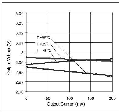
Fig.50 Load Regulation
