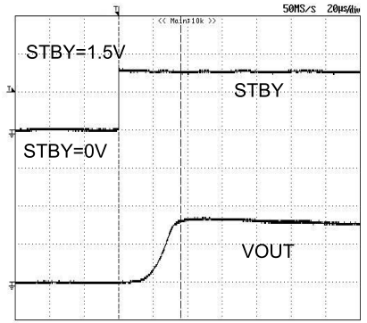
Fig.63 START_UP (Ta=85°C)
