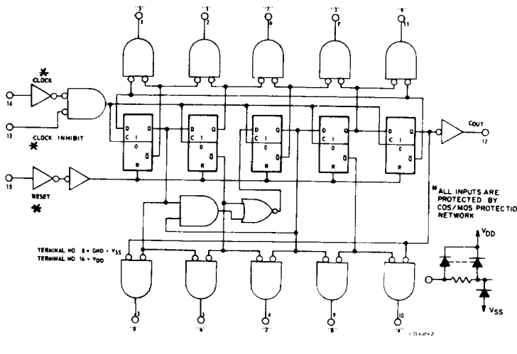
Fig. 1 - Logic diagram.
