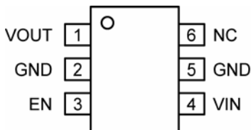
SC-70-6 (C6)
