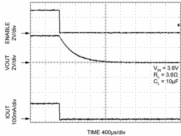
Turn-On/Turn-Off Timing
