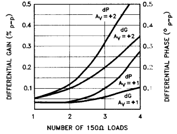
Differential Gain and Phase (30MHz)
