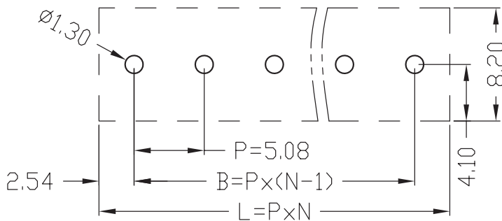
PCB LAYOUT
