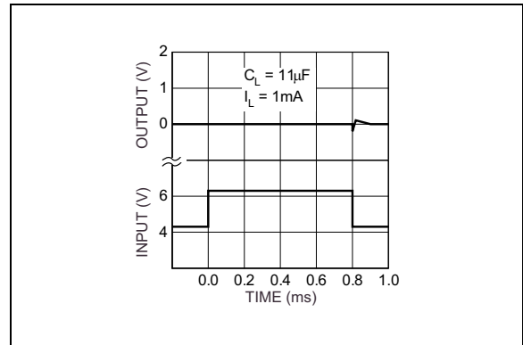
FIGURE 2-16: Line Transient.
