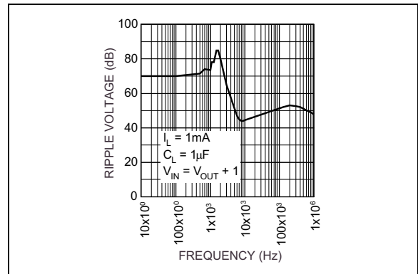
FIGURE 2-18: Ripple Voltage vs. Frequency.
