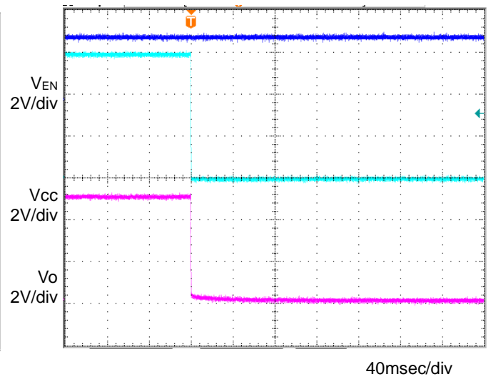
Fig.14 OFF sequence 1 Co=1μF,Ta=105°C
