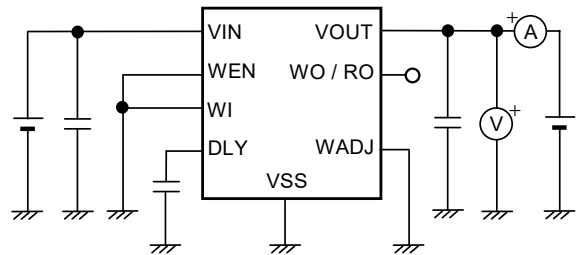
Figure 13 Test Circuit 2
