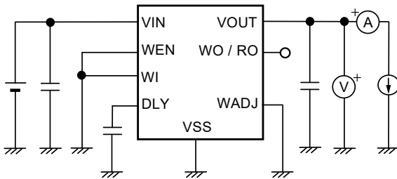
Figure 12 Test Circuit 1
