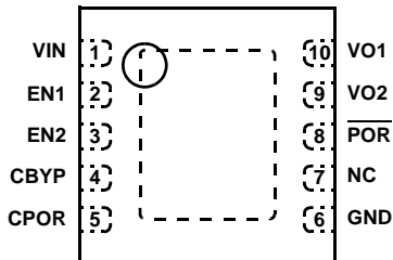
ISL9012 (10 LD 3X3 DFN) TOP VIEW
