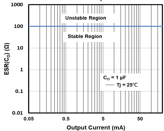
Figure 18. Output Capacitor Series Resistor ESR(C o ) vs. Output Current
