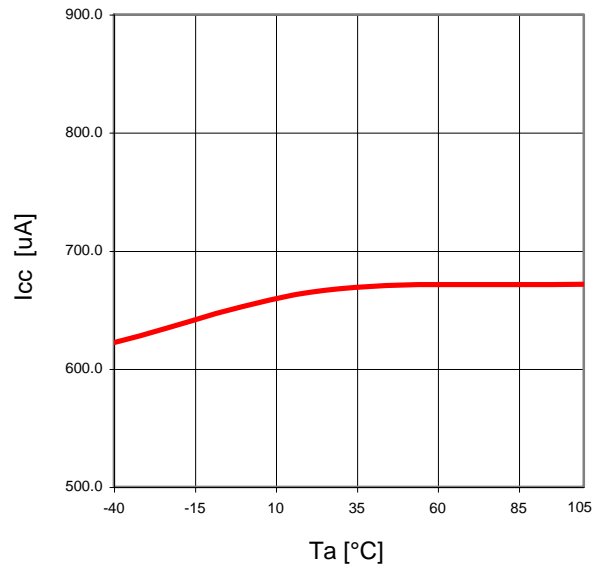
Fig.22 Ta-Icc
