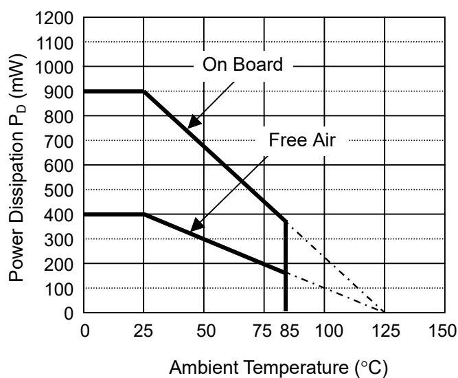
Power Dissipation
