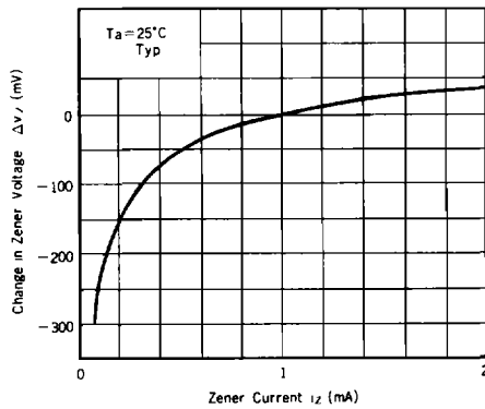
Fig. 5 ΔV Z - I Z Characteristic
