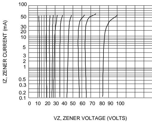
Fig. 3 BREAKDOWN CHARACTERISTICS (Vz = 12 - 82 V)
