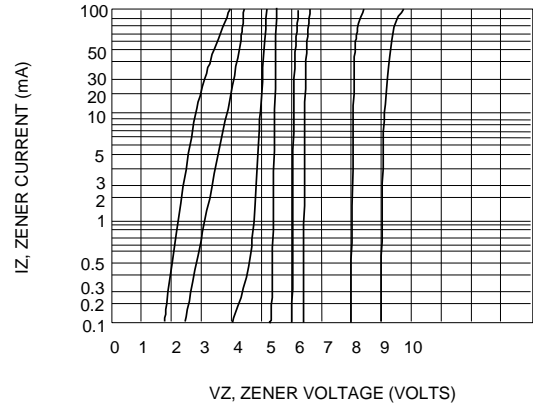
Fig. 2 BREAKDOWN CHARACTERISTICS (Vz = 3.9 - 10 V)
