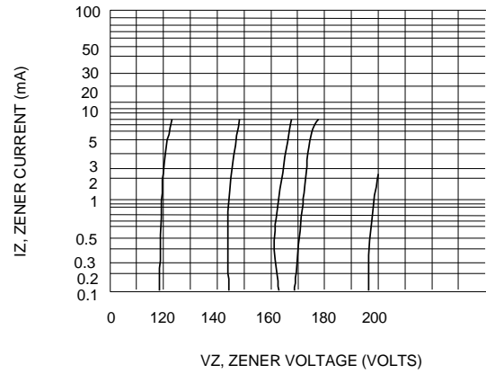
Fig. 4 BREAKDOWN CHARACTERISTICS (Vz = 100 - 200 V)
