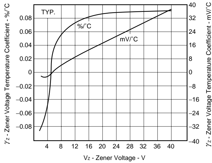
Figure 4. \gamma_z vs. V_z Example of Characteristics
