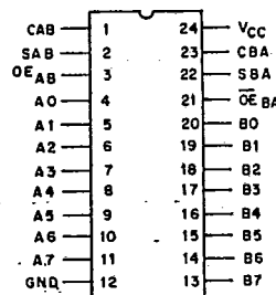
TERMINAL ASSIGNMENT 92CS-42678
