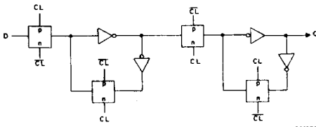
DETAIL OF TYPICAL D-TYPE M-S FLIP-FLOP
