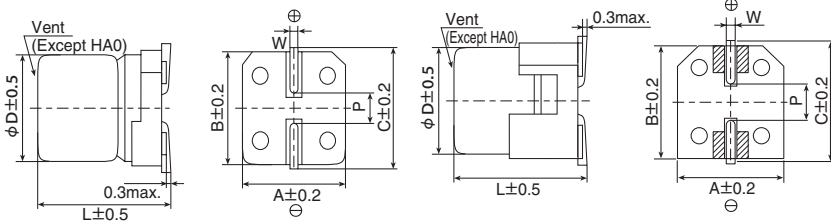
▨ : Dummy terminals
