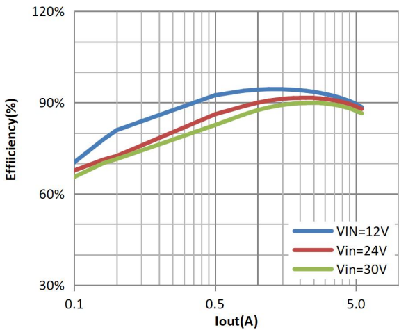
Efficiency & Iout (%)
