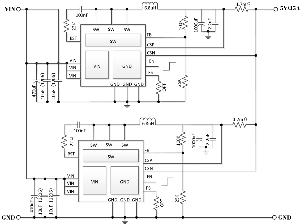
Dual Channel Power Supply
