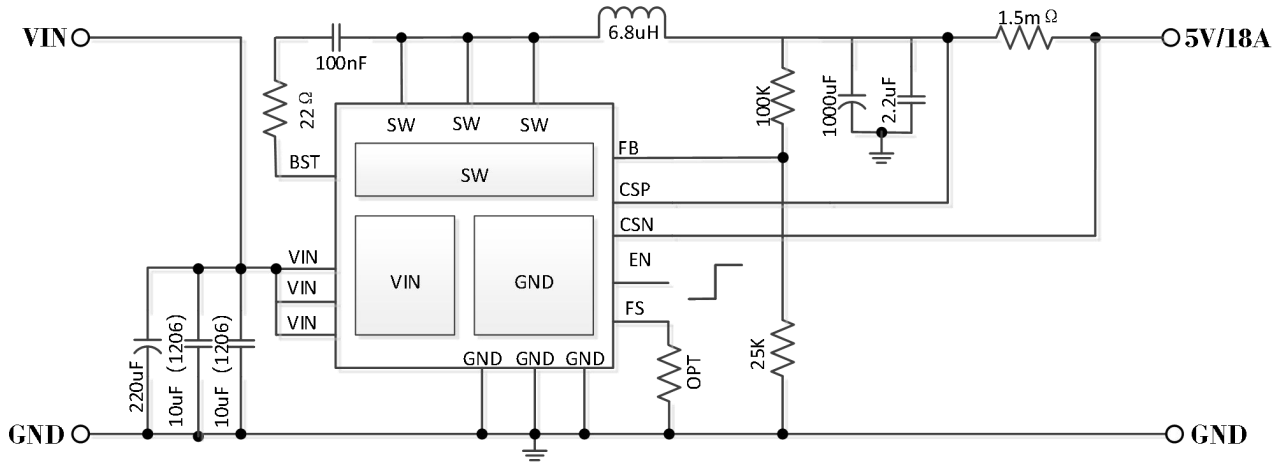
Single Channel Power Supply
