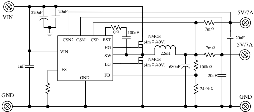
Dual Channel Application
