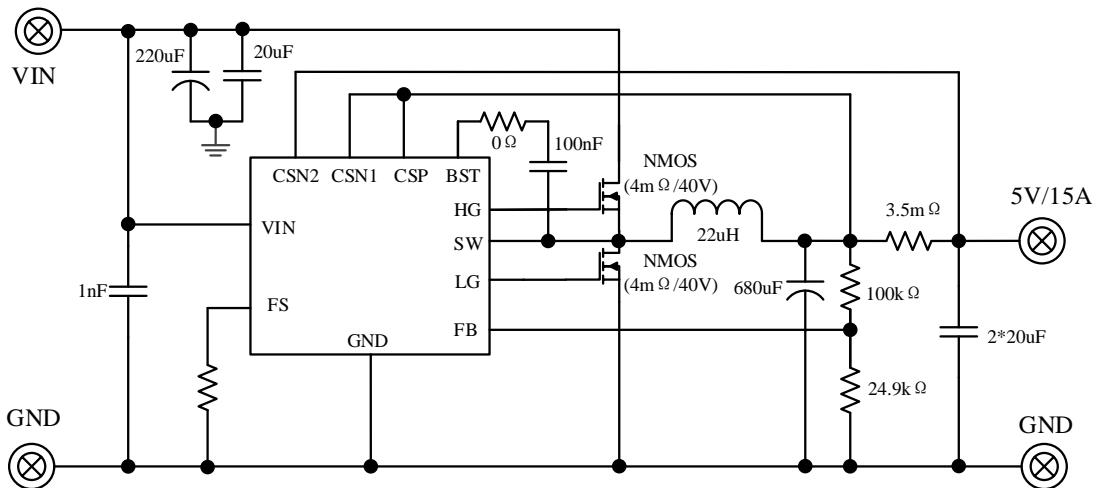
Single Channel Application
