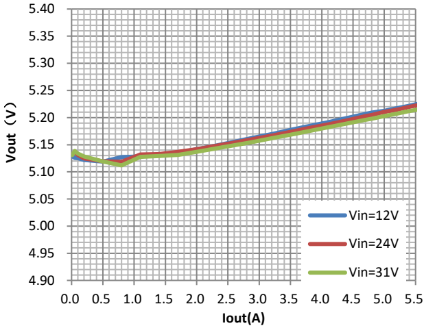
Line Regulation(Rupfb=100K)
