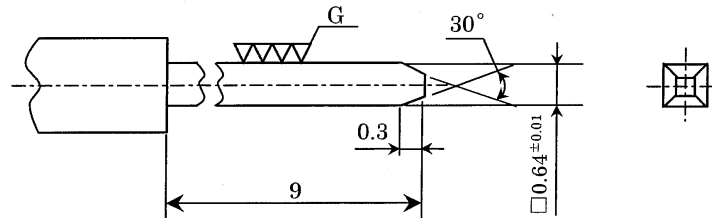
Fig. 1 Configuration and Dimensions of Steel Gauge
