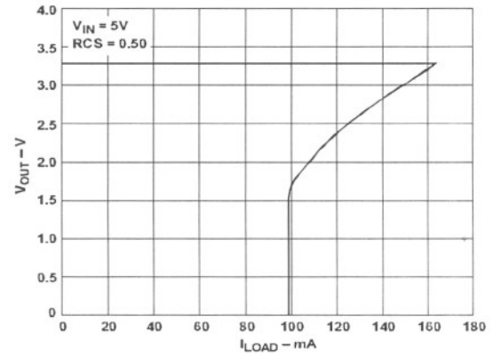
Figure 13. Foldback Current
