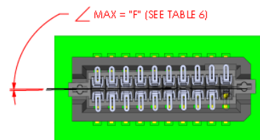
FINAL Z AXIS ANGULAR MISALIGNMENT
