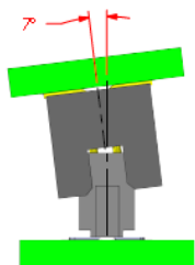
INITIAL X AXIS ANGULAR MISALIGNMENT
