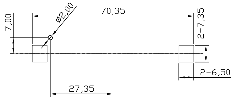
MOUNTING DETAIL
