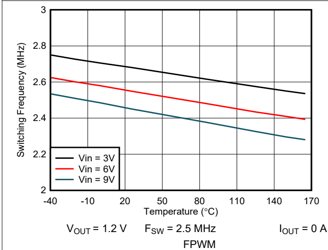
图 7-11. Switching Frequency vs Temperature
