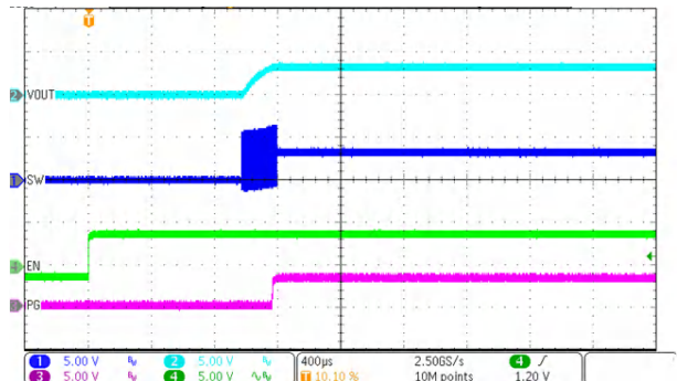
图 9-65. Start-Up Timing
