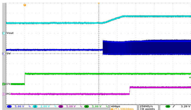
图 9-66. Start-Up Timing
