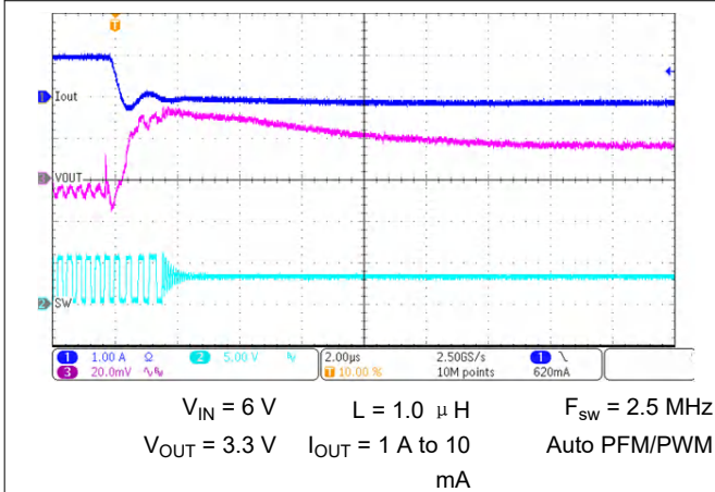
图 9-74. Load Transient Response Overshoot
