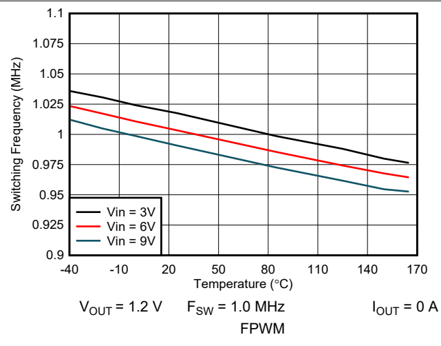
图 7-12. Switching Frequency vs Temperature
