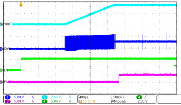
图 9-64. Start-Up Timing
