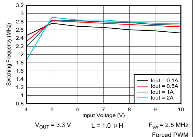
图 9-55. Switching Frequency vs Input Voltage
