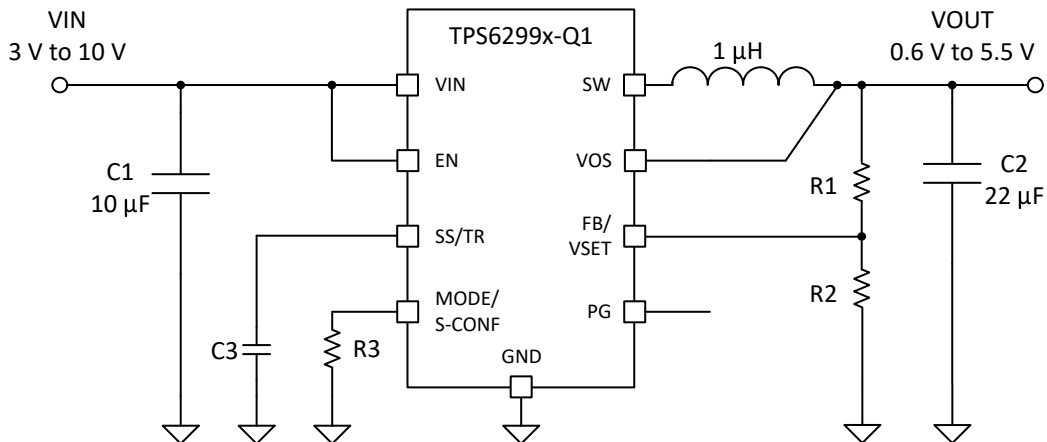
图 8-2. Adjustable V O Operation Schematic
