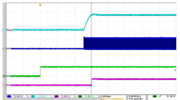
图 9-65. Start-Up Timing
