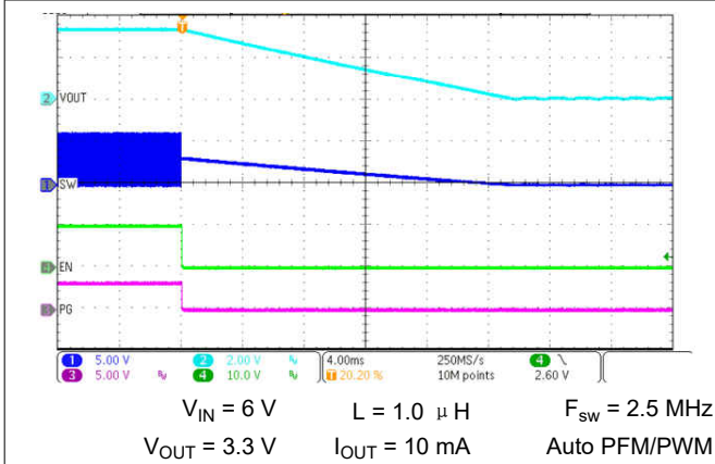
图 9-70. Shutdown Timing with Output Discharge Disabled
