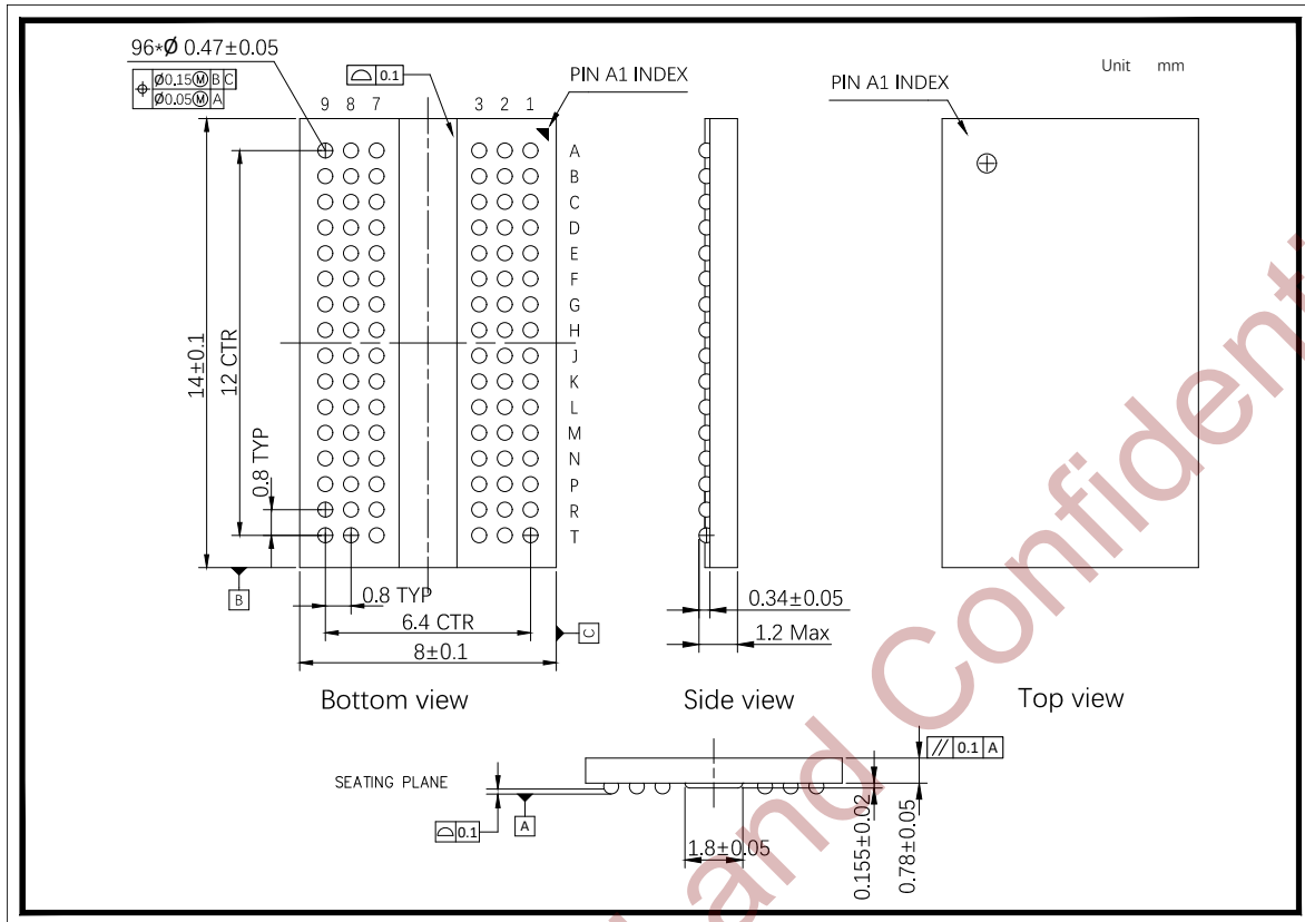
Figure 2-2 96-Ball FBGA - x16 Component
