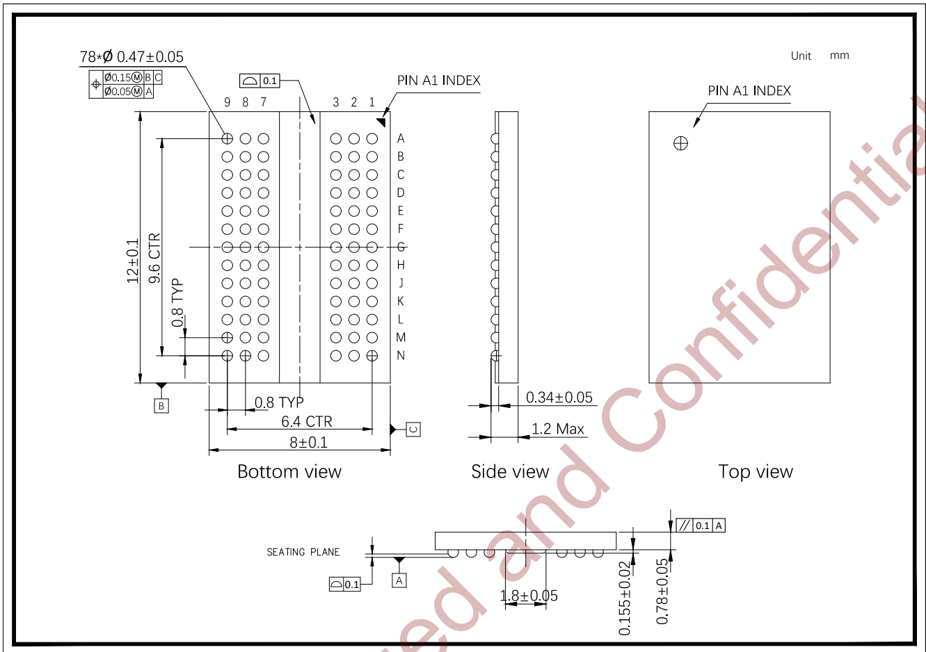
Figure 2-1 78-Ball FBGA - x8 Component
