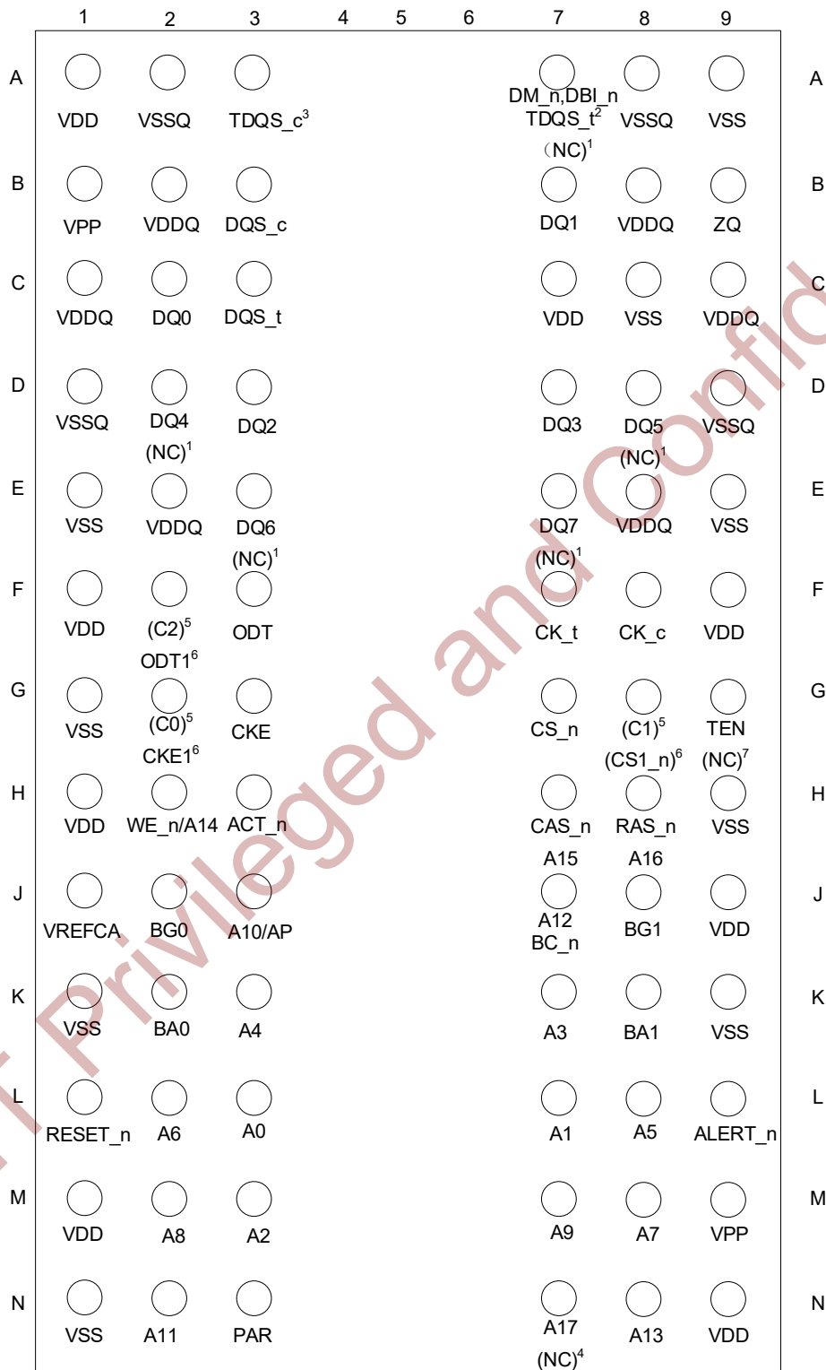
Figure 2-3 DDR4 Ball Assignments for the x8 Component
