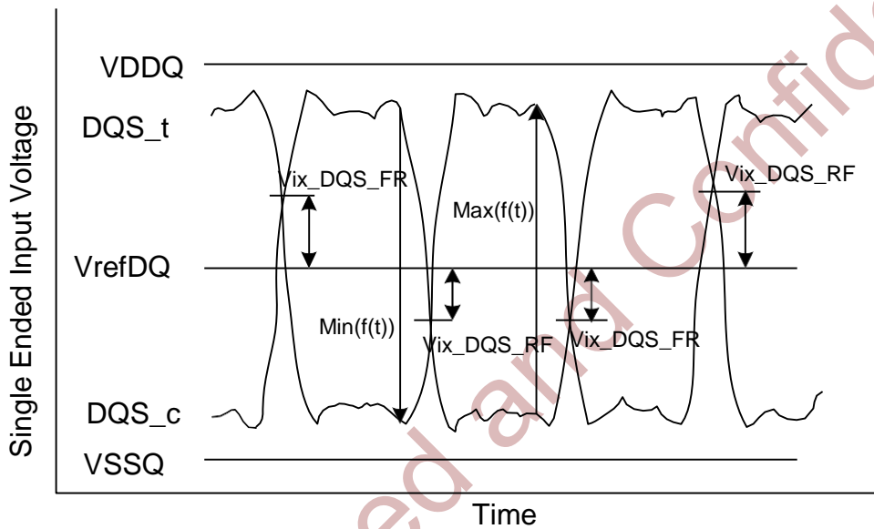
Figure 5-15 Vix Definition (DQS)
