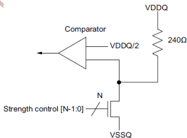
Figure 5-19 Pull-down Calibration
