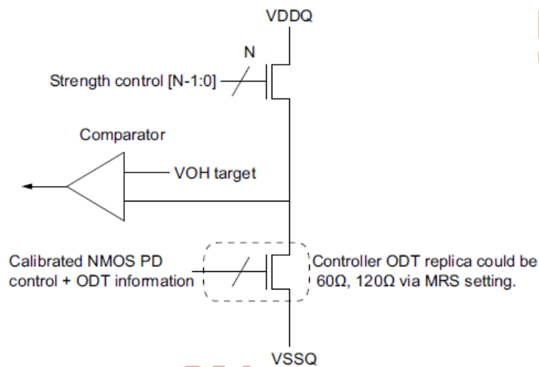
Figure 5-20 Pull-up Calibration
