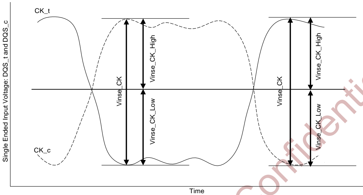
Figure 5-8 Clock Single-Ended Input Voltage
