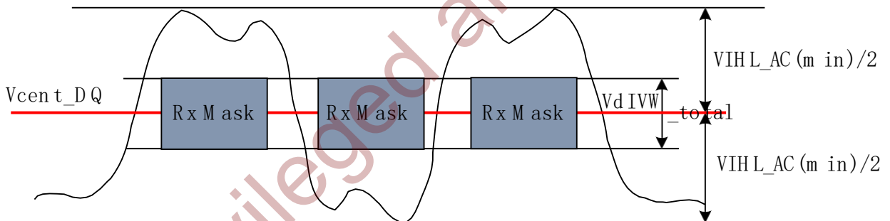
Figure 8-32 DQ VIHL\_AC definition (for Each Input Pulse)
