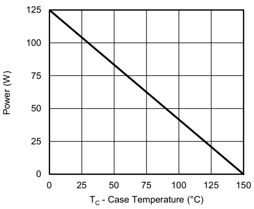
Power, Junction-to-Case
