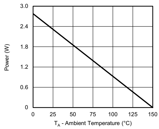
Power, Junction-to-Ambient
