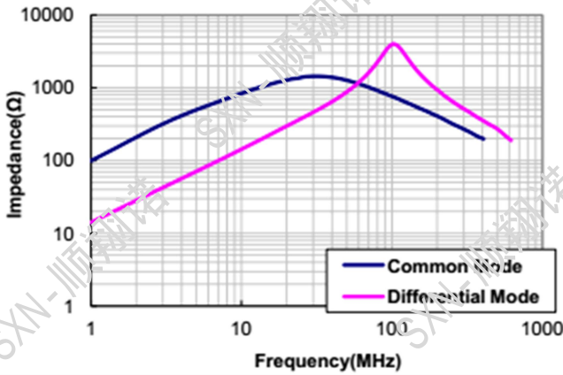
SMCM1211-222T
