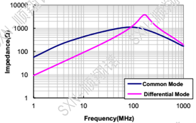
SMCM1211-102T
