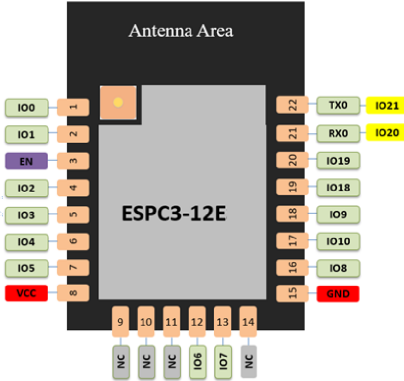
Fig.2.1 ESPC3-12E Pins Definition
