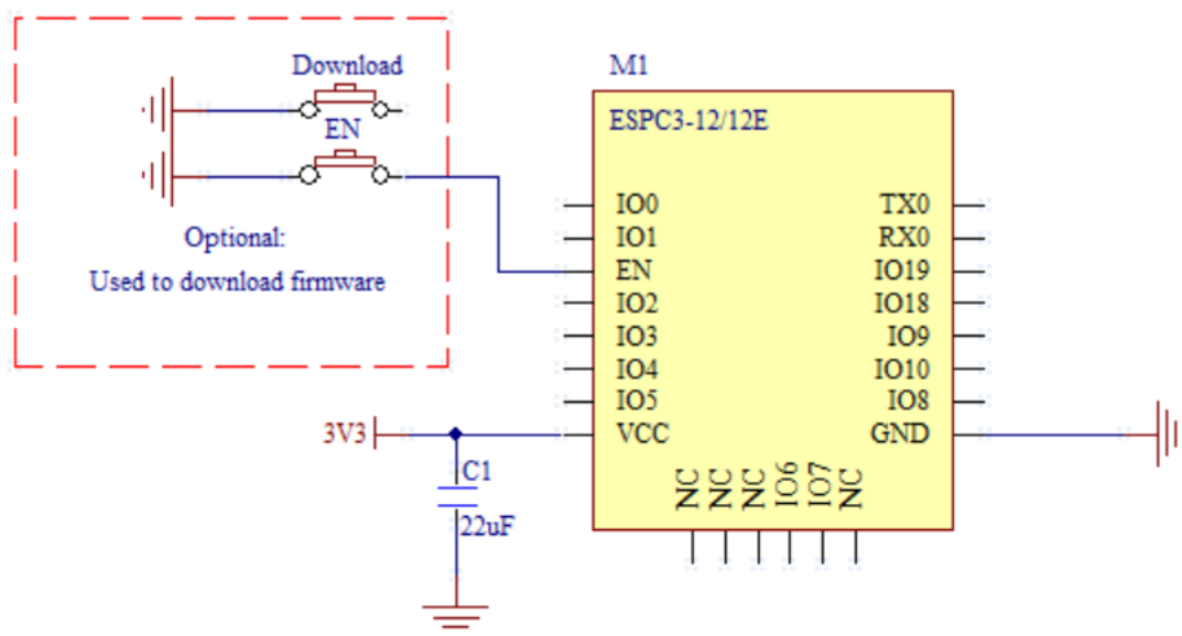
Fig.9.1 Minimum System
