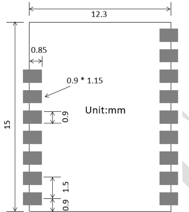
Fig. 3.3 PCB Layout for ESP-M1
