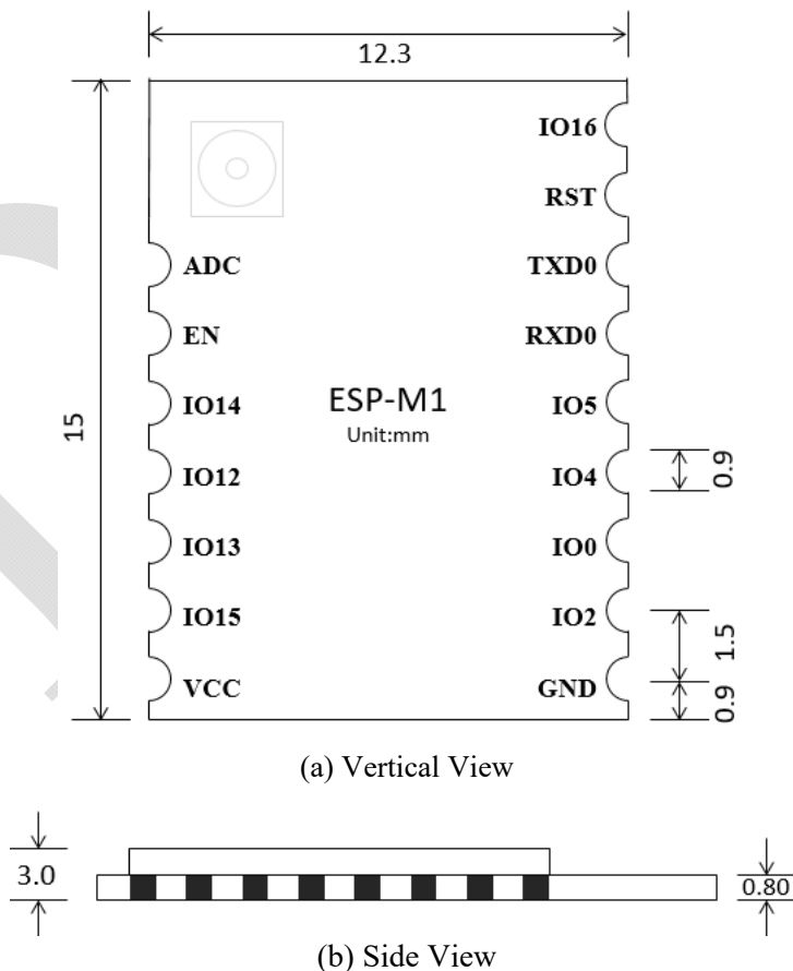
Fig. 3.2 Size for ESP-M1
