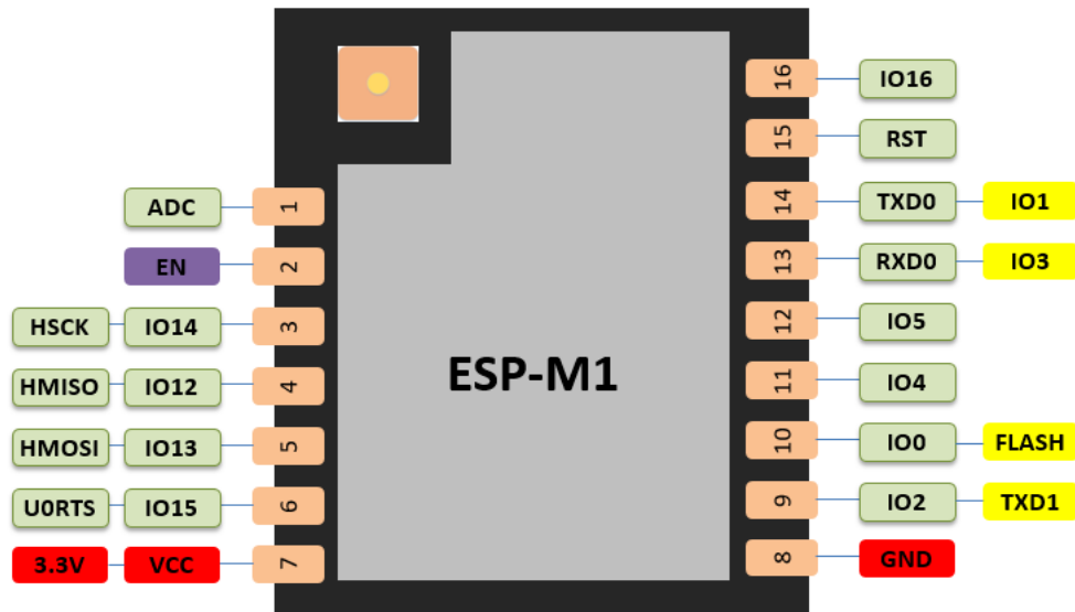
Fig. 2.1 ESP-M1 Pins Definition
