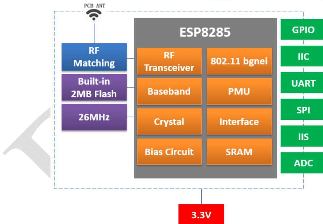
Fig. 1.1 DT-LIGHT Module Structure
