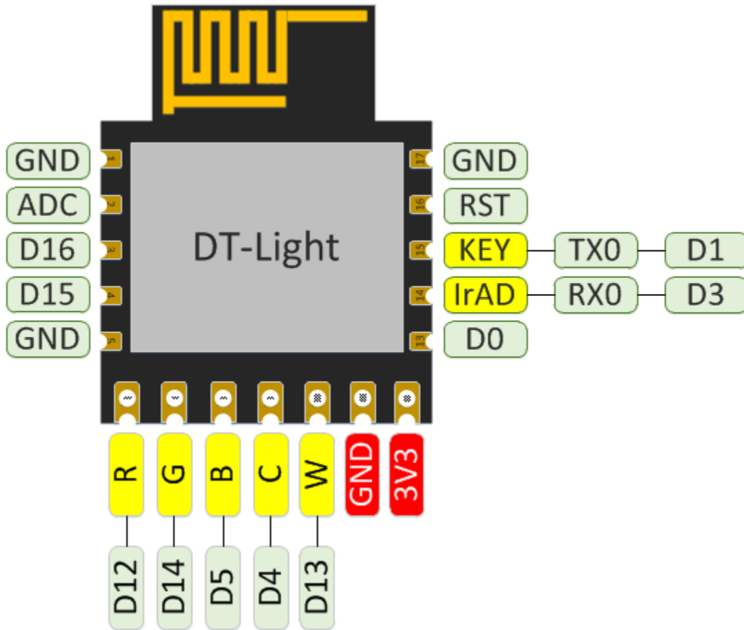
Fig. 2.1 DT-LIGHT Pins Definition
