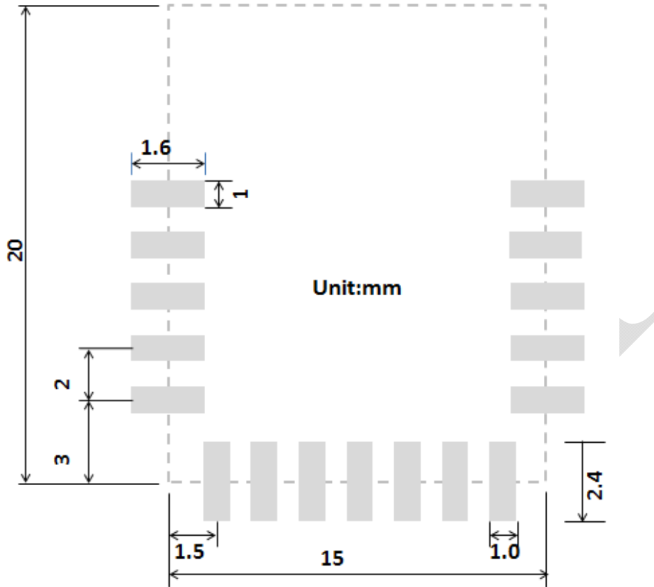
Fig. 3.3 PCB Layout for DT-LIGHT
