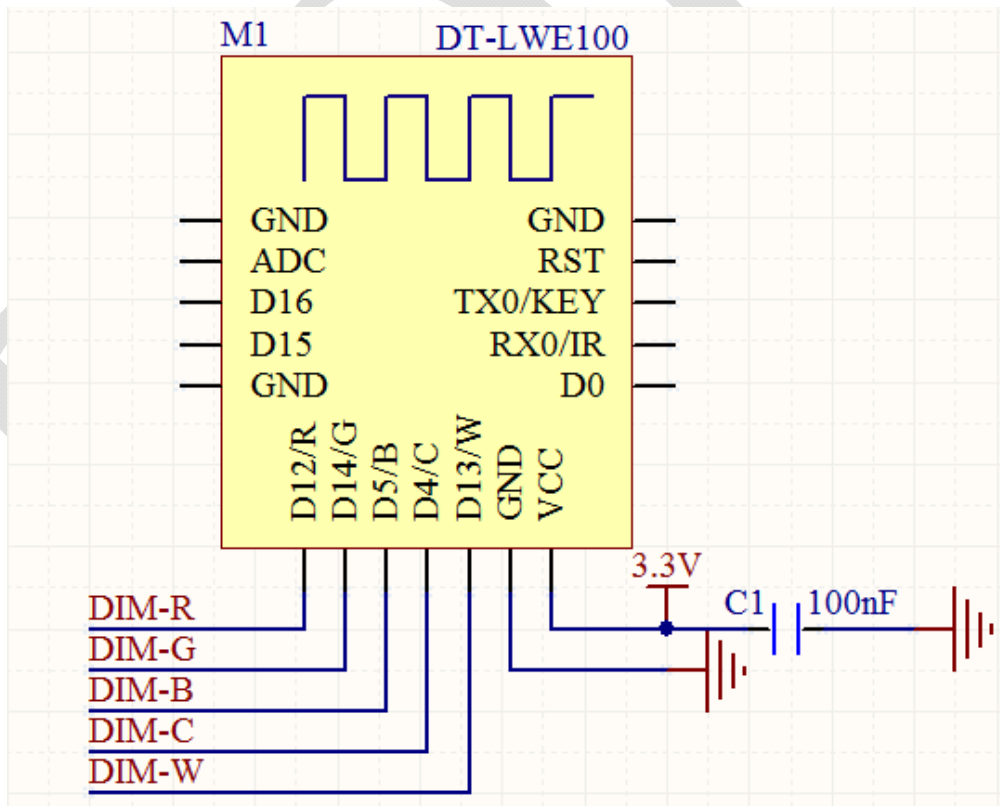
Fig.8.1 Minimum user system
