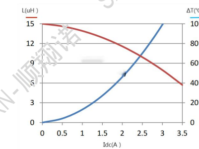
SMMS0518-150M
