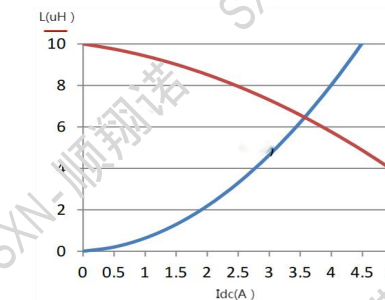
SMMS0518-100M
