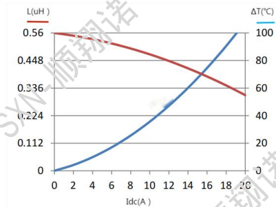
SMMS0518-R56
