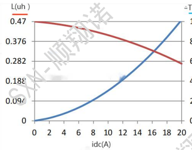
SMMS0518-R47M
