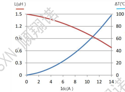
SMMS0518-1R5M
