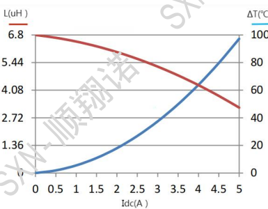
SMMS0518-6R8M
