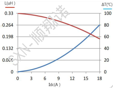
SMMS0518-R33M
