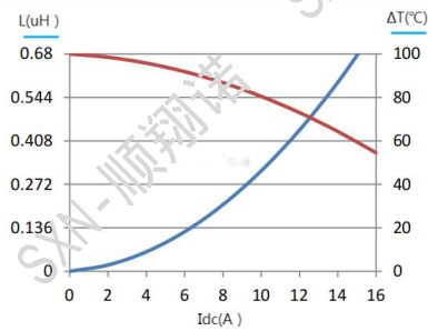
SMMS0518-R63M
