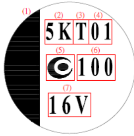
Fig. 3 Marking
