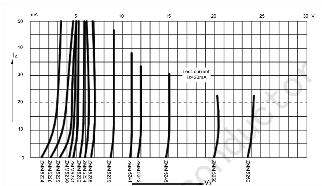
FIG.1 -- BREAKDOWN CHARACTERISTICS
