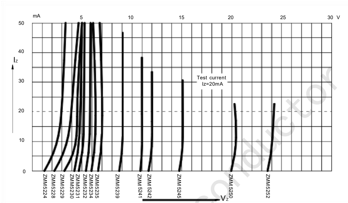
FIG.1 -- BREAKDOWN CHARACTERISTICS
