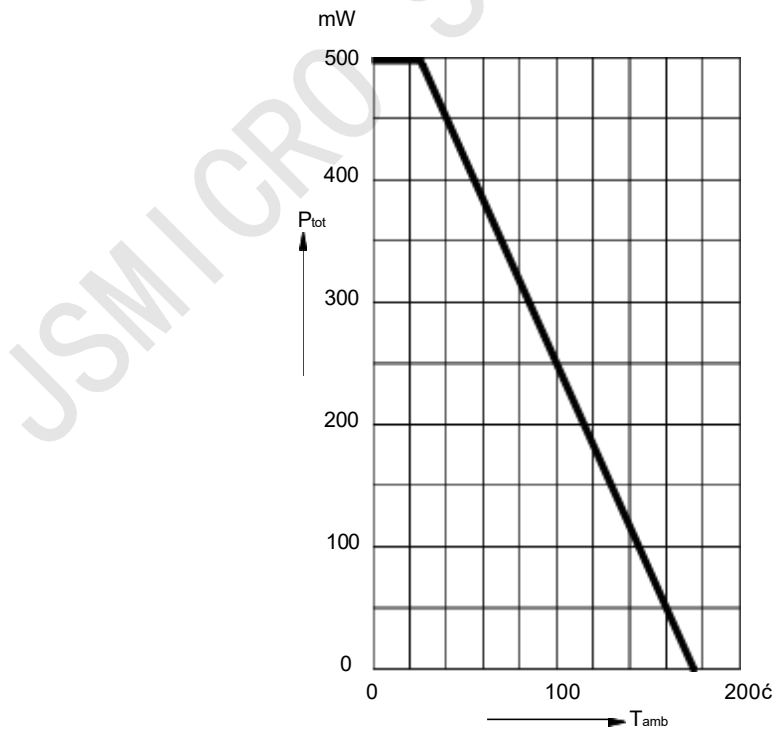
FIG.2 -- ADMISSIBLE POWER DISSIPATION VERSUS AMBIENT TEMPERATURE
