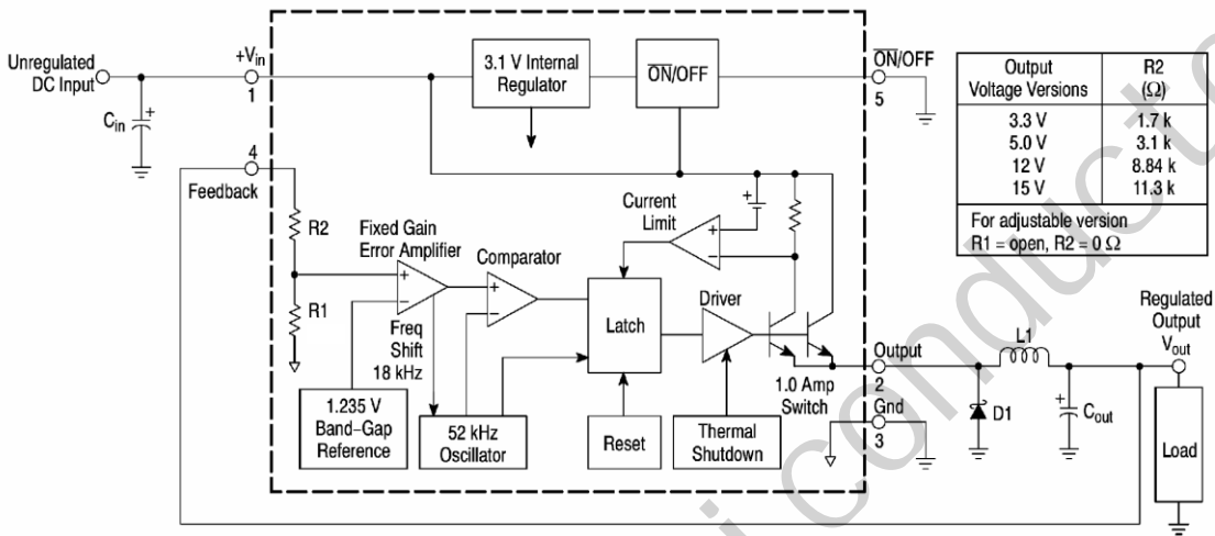
Representative Block Diagram and Typical Application
