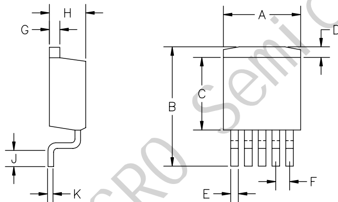
Outline Drawing:TO-263-5
