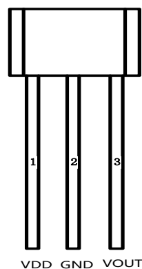
TO92S
