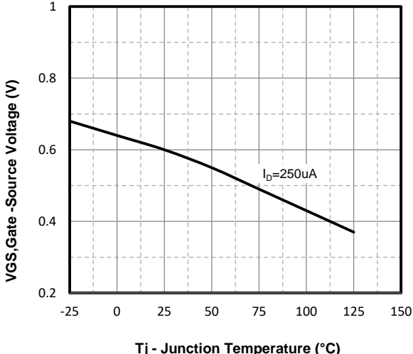
Fig3. Normalized Threshold Voltage Vs. Temperature
