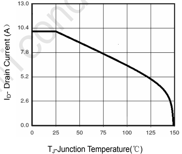
Figure 4 Drain Current
