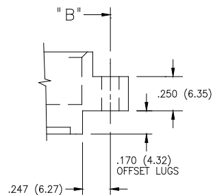
IN-CONTACT POLARIZING KEY P/N 345-240-328
