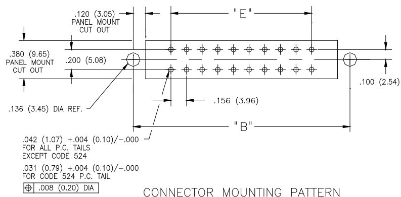
RECOMMENDED DAUGHTER BOARD
