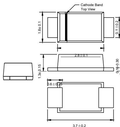
SOD-123FL
