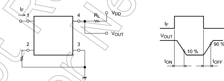
Fig. 11.1 Switching Time Test Circuit and Waveform
