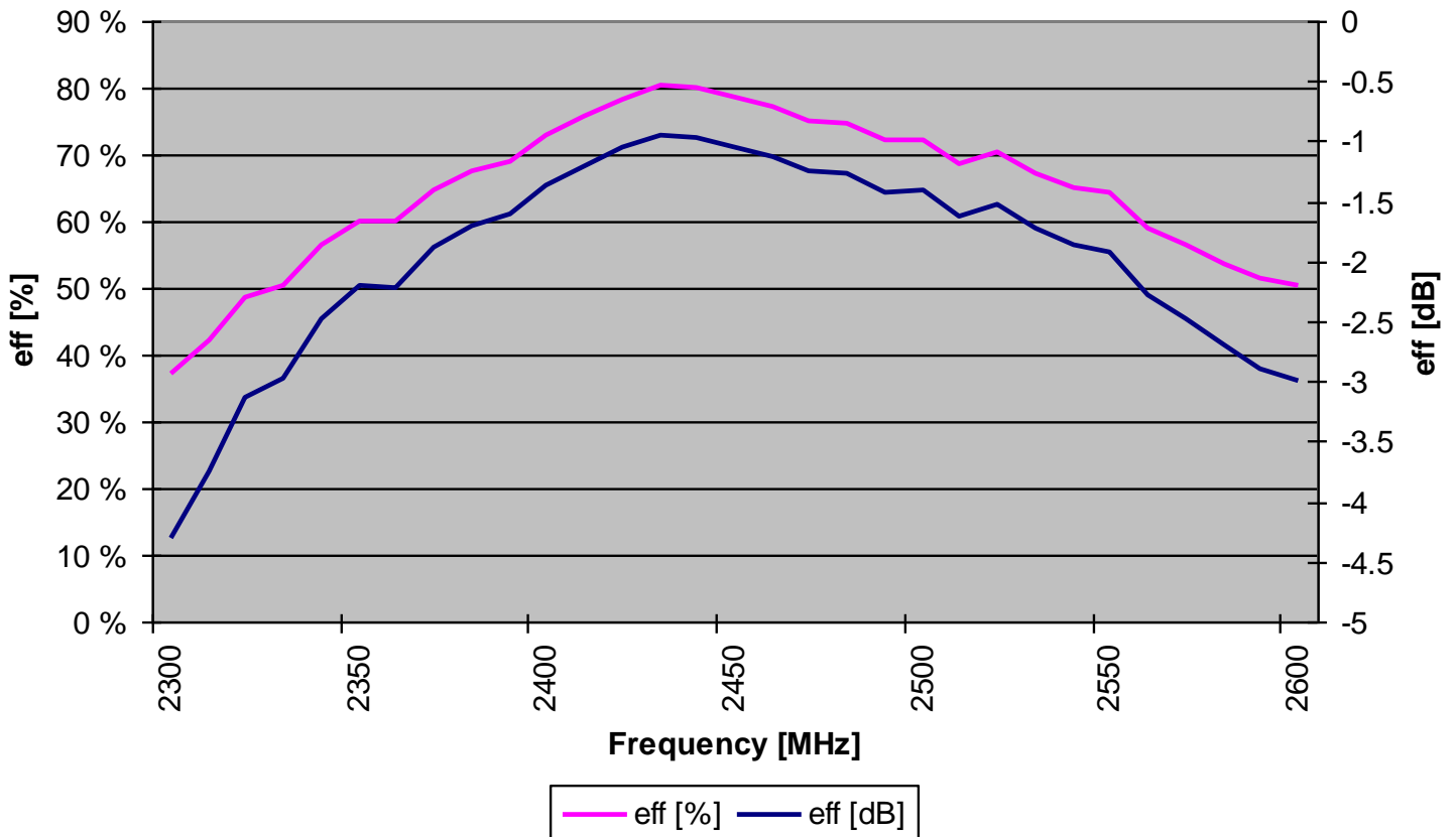
W3064C BT total antenna efficiency
